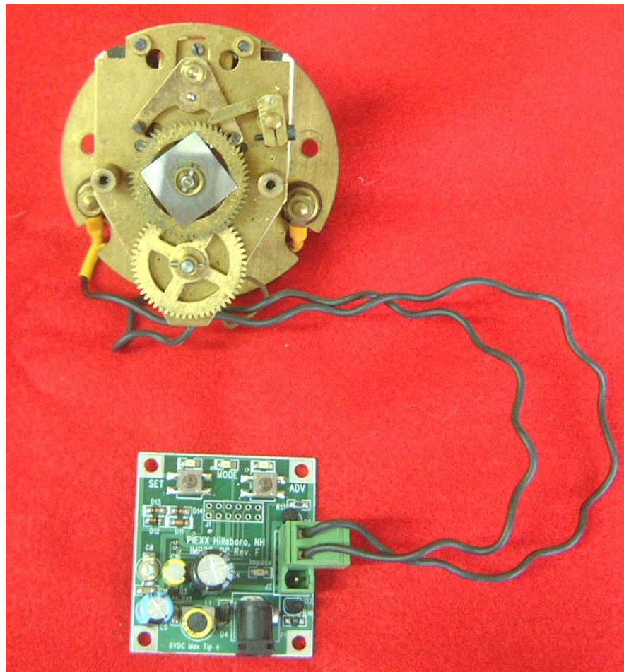
IMP-22 Connected to a Brille Movement. Brille uses the same connections as a Gents.
