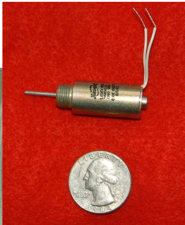
A 24VDC Solenoid mounted inside of a 4" Bell for Hour Strike
