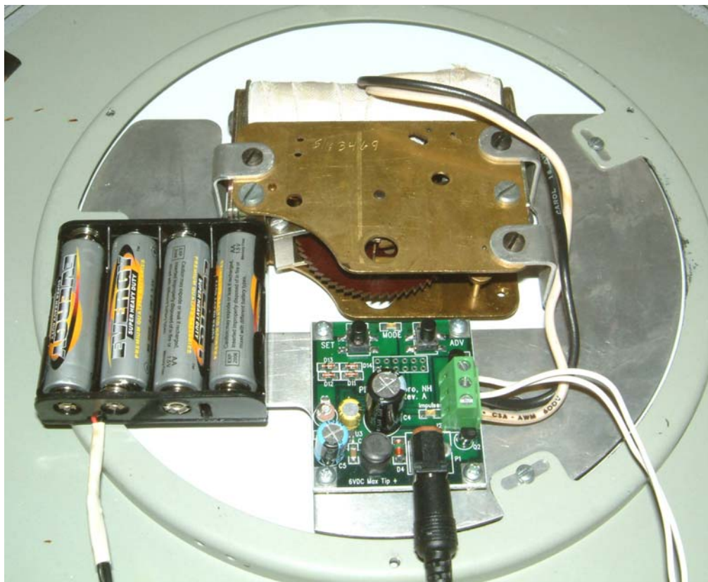
IMP-2 Inside Stromberg Clock. The 2 white wires connect to the strike mechanism.
