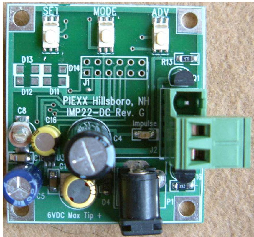
The IMP-22G is only 2.05" x 1.85"
